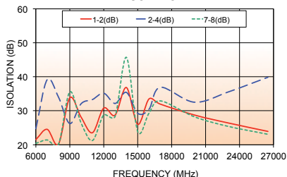
ZC8PD-06263+ ISOLATION
