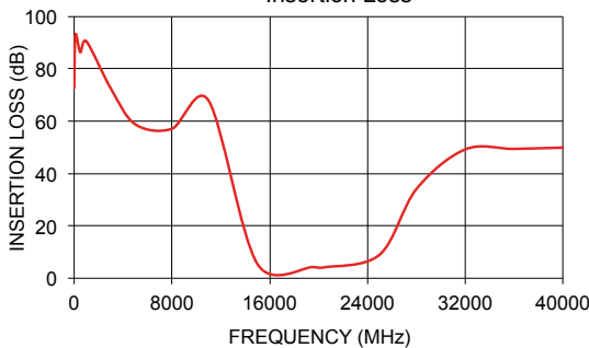
Insertion Loss
