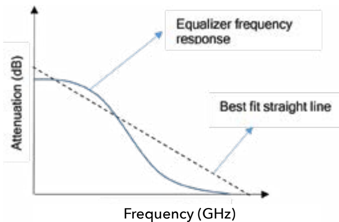
Figure 3: Negative slope equalizer
