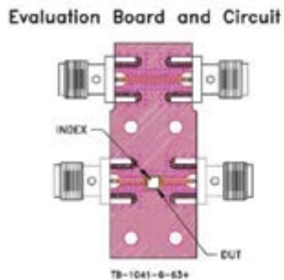
Figure 9b: Evaluation board for EQY-6-63+
