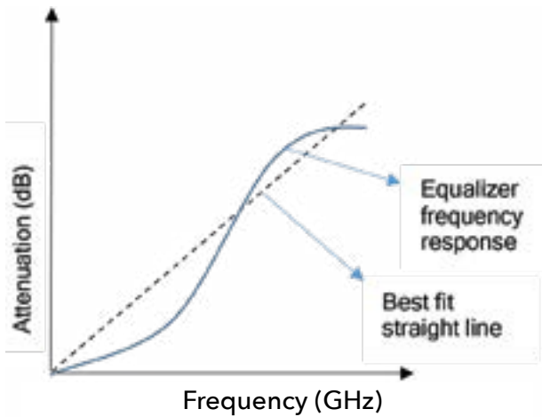
Figure 2: Positive slope equalizer
