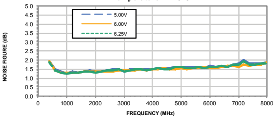
NOISE FIGURE vs. FREQUENCY & DEVICE VOLTAGE Temperature = +25°C
