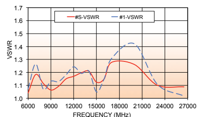
ZC8PD-06263+ VSWR
