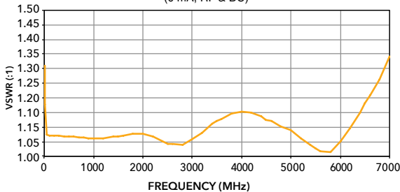
VSWR (0 mA, RF & DC)
