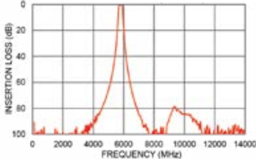
ZVBP-5800+ Insertion Loss (Full Band)
