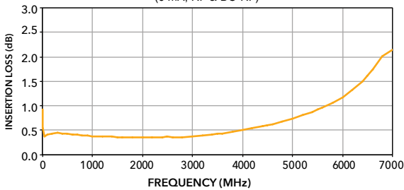
INSERTION LOSS (0 mA, RF & DC-RF)
