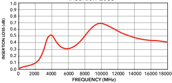
Insertion Loss
