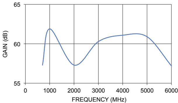
ZHL-50W-63+ GAIN
