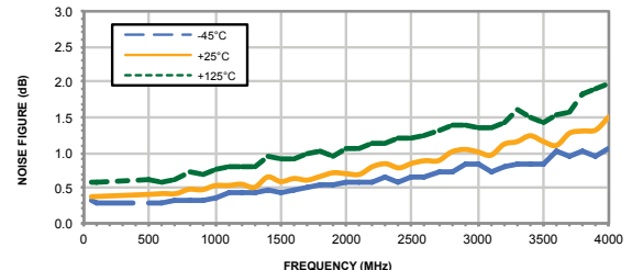
NOISE FIGURE vs. FREQUENCY & DEVICE VOLTAGE Vd = 5.00V
