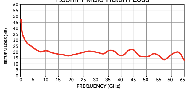
1.85mm-Male Return Loss
