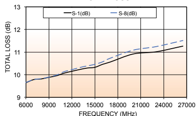
ZC8PD-06263+ TOTAL LOSS
