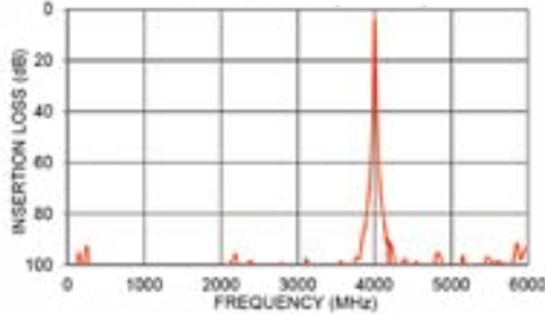
ZVBP-4000+ Insertion Loss ( Full Band)
