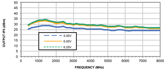
OUTPUT IP3 vs. FREQUENCY & DEVICE VOLTAGE OUTPUT POWER = 0.00dBm, Temperature = +25°C
