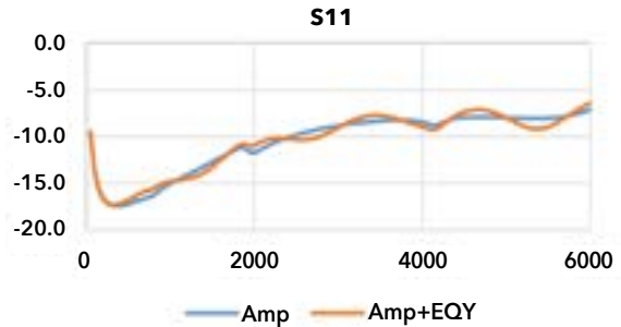
Figure 13: Comparison of input return loss for amplifier alone vs. amplifier-equalizer combination.
