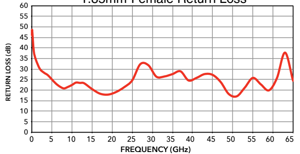
1.85mm-Female Return Loss
