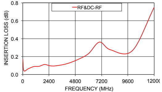
INSERTION LOSS
