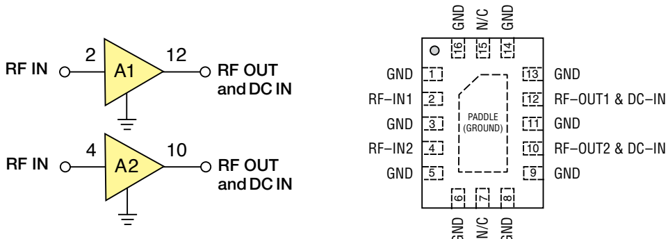
Simplified schematic (each of A1, A2) and pad description
