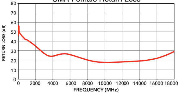
SMA-Female Return Loss
