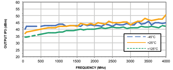
OUTPUT IP3 vs. FREQUENCY & TEMPERATURE OUTPUT POWER = 5.00dBm, Vd = 5.00V
