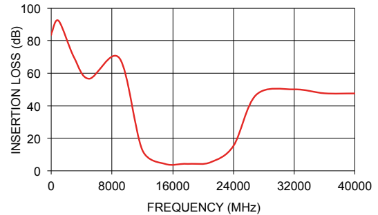
Insertion Loss
