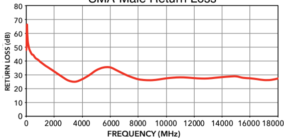
SMA-Male Return Loss
