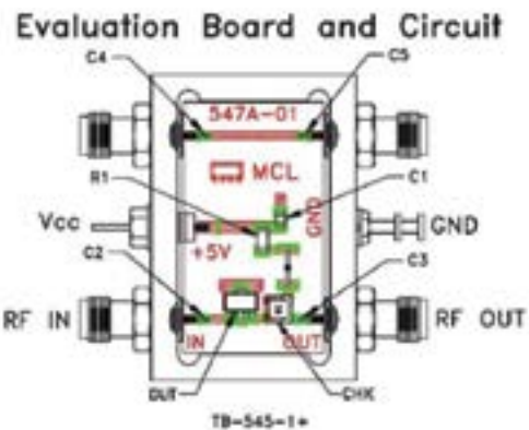
Figure 9a: Evaluation board for PHA-1+ MMIC Amplifier
