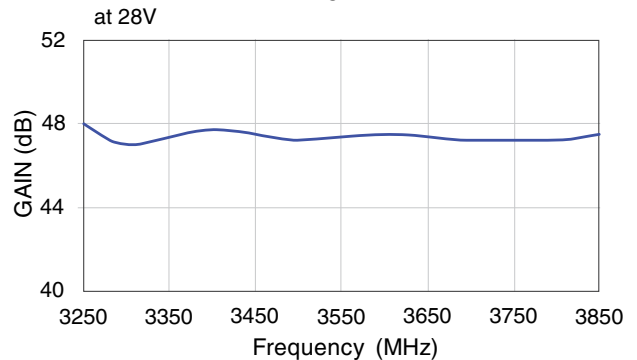
ZHL-100W-382+ GAIN
