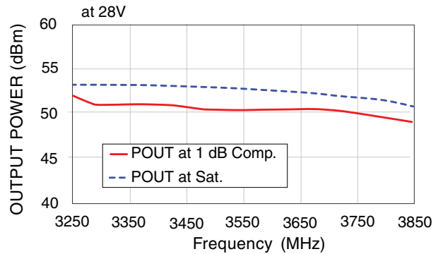
ZHL-100W-382+ OUTPUT POWER
