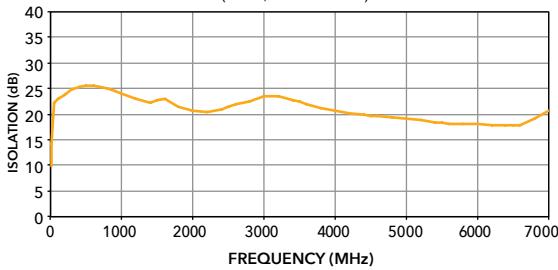
ISOLATION (0 mA, RF & DC-DC)
